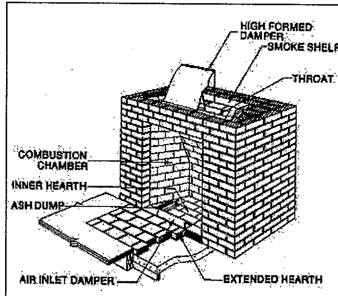
Typical Firebox Assembly
