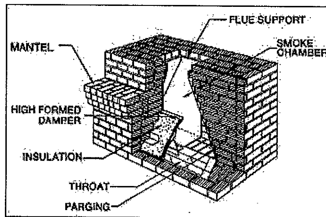
Typical Smoke Chamber Assembly
