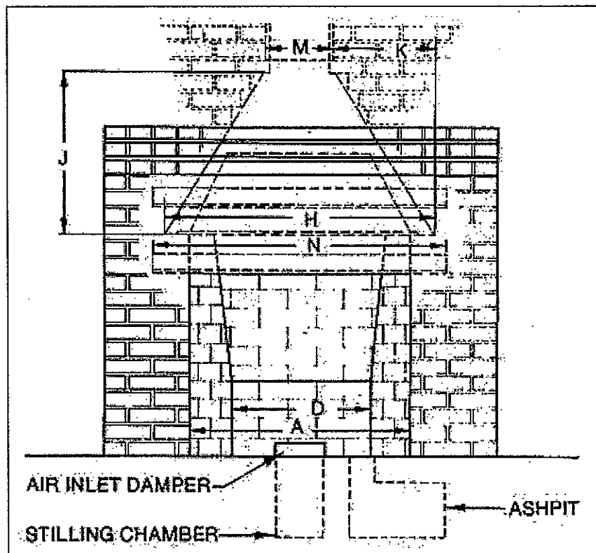
Typical Single-Face Fireplace (See Table 1 for Dimensions)
