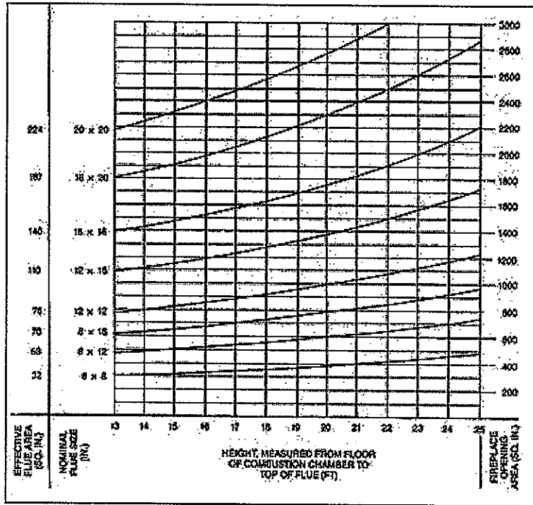
Flue Size Nomograph
