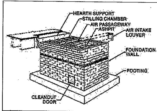
Typical Base Assembly
